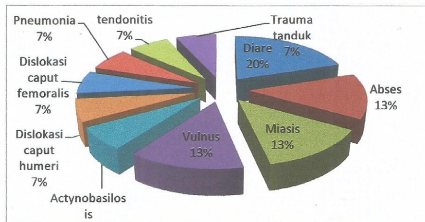
Diagram 1. Persentase kasus bulan September 2020
